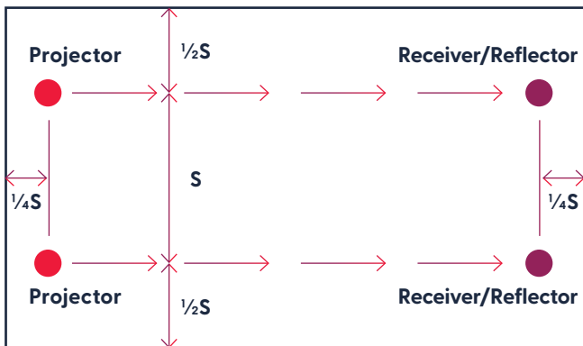
Figure A17.7.4.7: Maximum distance at which ceiling suspended light Projector and Receiver/Reflector can be positioned from end wall is one quarter selected spacing ( S )
